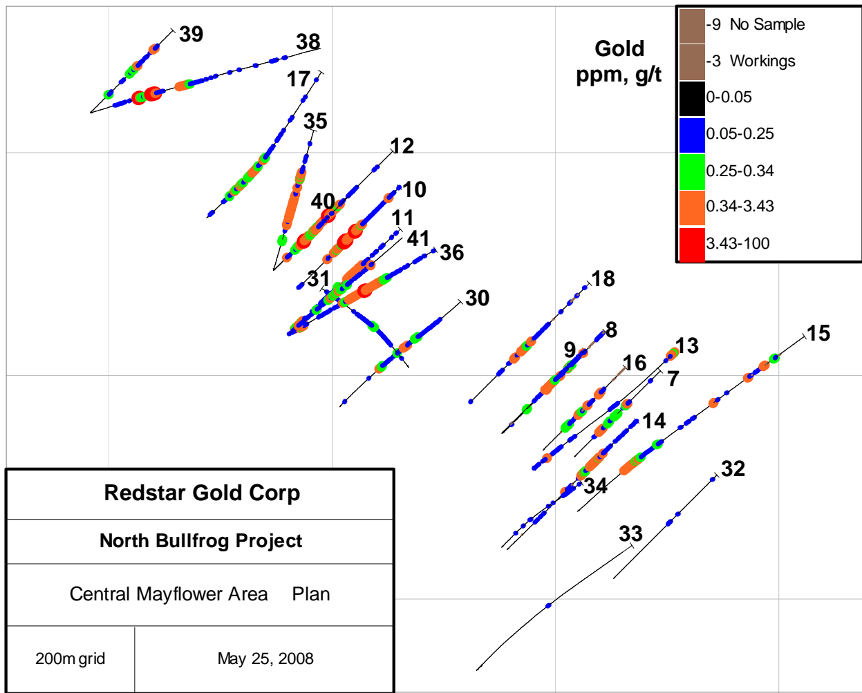
Plan of the central Mayflower deposit showing drill holes completed in 2008 (NB-08-#).
